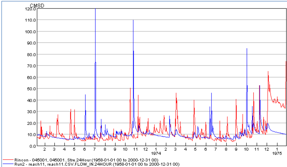
Figure 6-14. Rincon observed (red) and simulated (blue) streamflow
