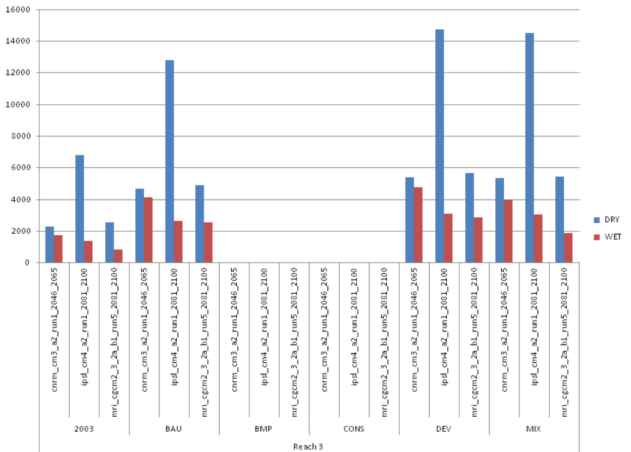
Figure 7-6. Seasonal variation of sediment load in reach 3 of the Haina basin for the dry and wet seasons.
