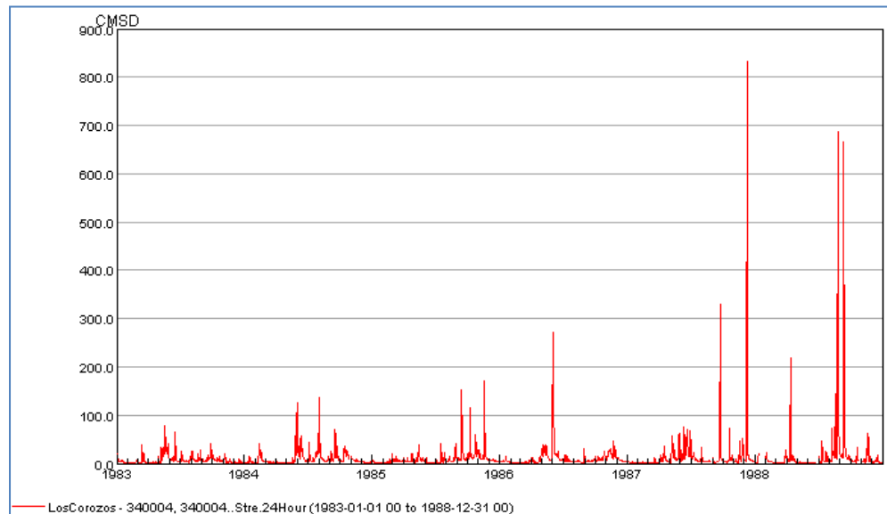
Figure 6-7. Los Corozos streamflow data
