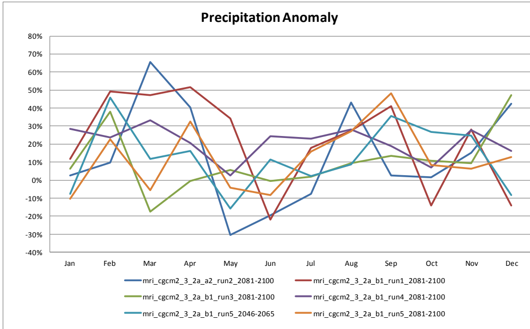
Figure 5-15. Monthly percent change in precipitation for the selected climate change projections in the wet and warm climate zone.
