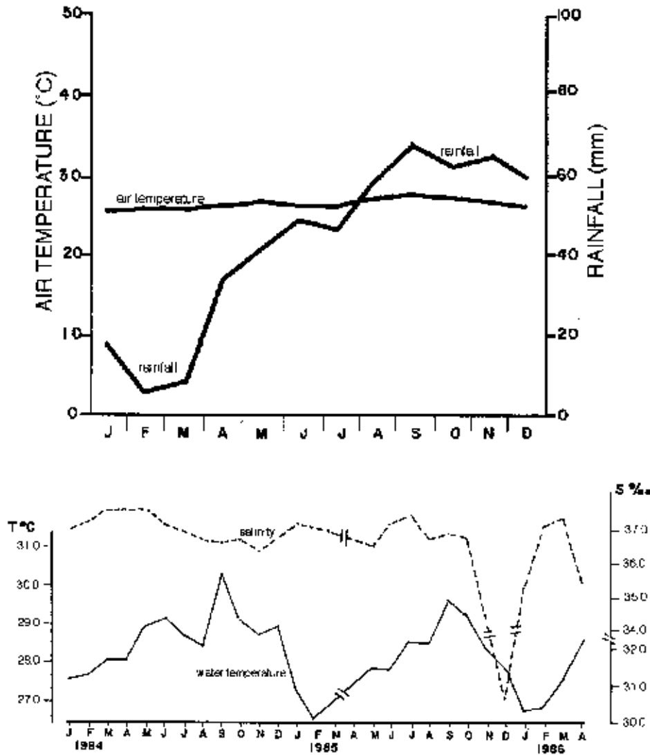
Fig. 2. Annual air temperature and rainfall pattern (top) and annual water temperature and salinity fluctuations (bottom) at Punta Murín, Morón, Golfo Triste.
