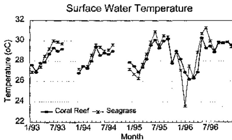
Fig. 4. Surface (0.5 m depth) water temperature over the drop-off seaward of Carrie Bow Cay and at CARICOMP Seagrass Site U; monthly mean from January 1993 to December 1996.
