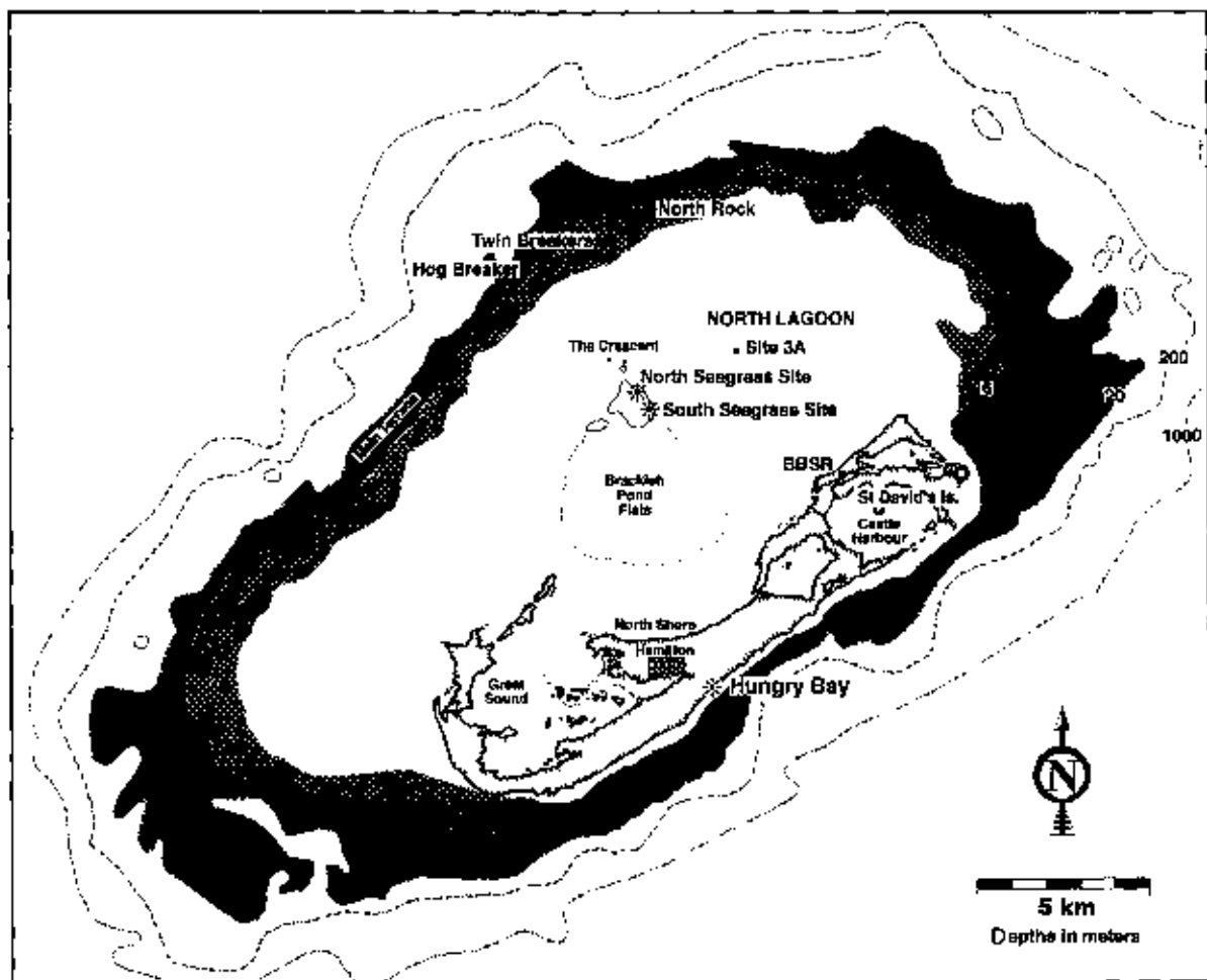
Fig. 1. Map of the Bermuda Platform, showing the outer reef zones surrounding the central North Lagoon, which contains numerous patch reefs (e.g., Brackish Pond Flats and the Crescent) and muddy depressions. The CARICOMP study sites are marked with the symbol *. The site for climatic data collection on St. David's Island marked with the symbol C.
