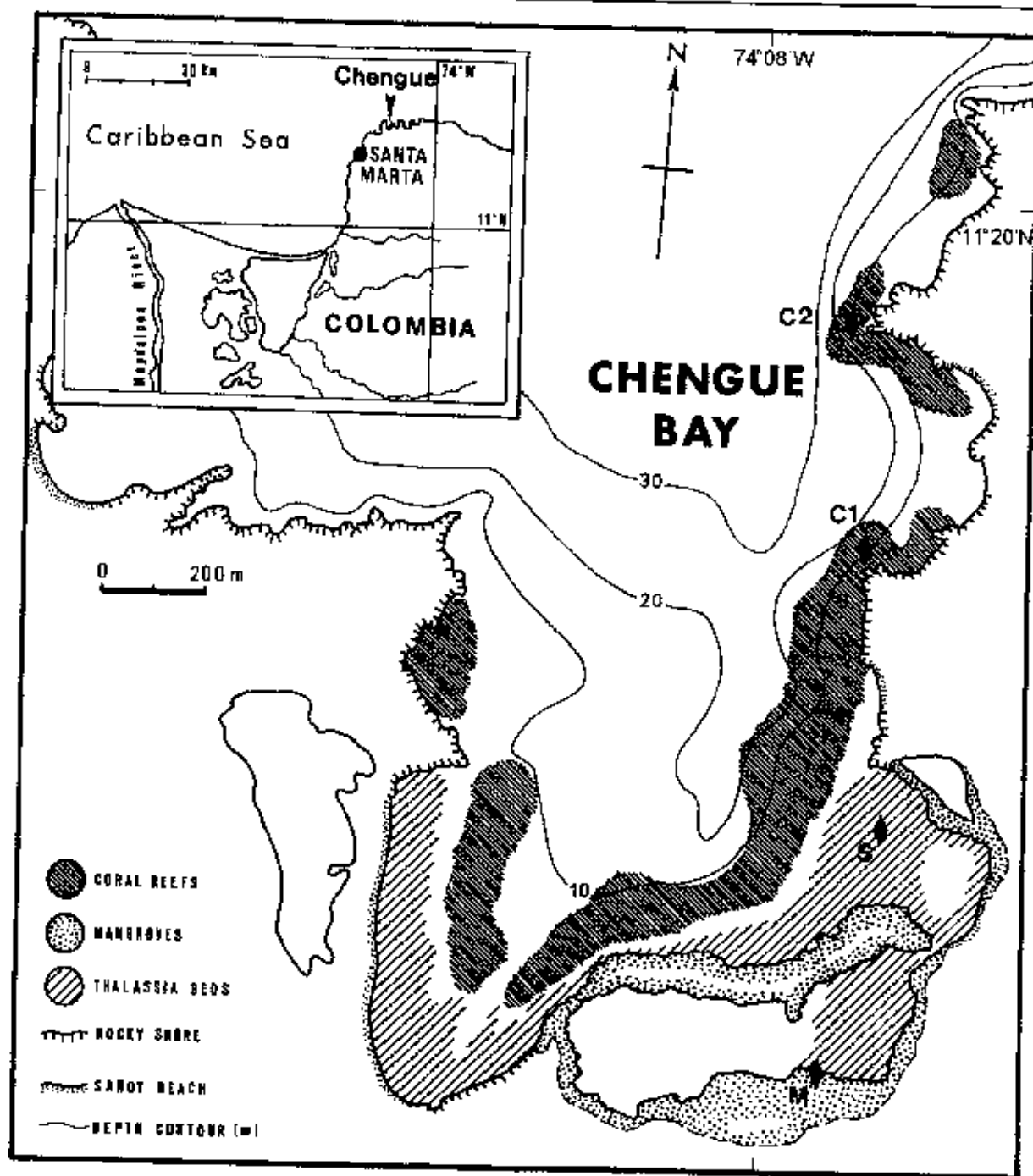
Fig. 1. Map of Bahía de Chengue, indicating bathymetry, distribution of principal coastal marine ecosystems, location of CARICOMP sampling sites (black diamonds): mangrove wetlands (M), seagrass beds (S), and coral reefs (C1 and C2). Coral reef physical measurements were taken at site C1. Inset map includes a section of the Caribbean coast of Colombia, showing the locations of Bahía de Chengue, Santa Marta, and the mouth of the Magdalena River.
