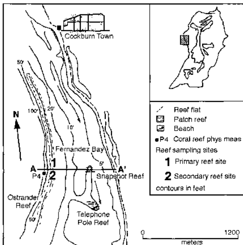
Fig. 8. Coral reef sampling site in Fernandez Bay, western coast of San Salvador, Bahamas. Section A-A' is displayed in Fig. 9.
