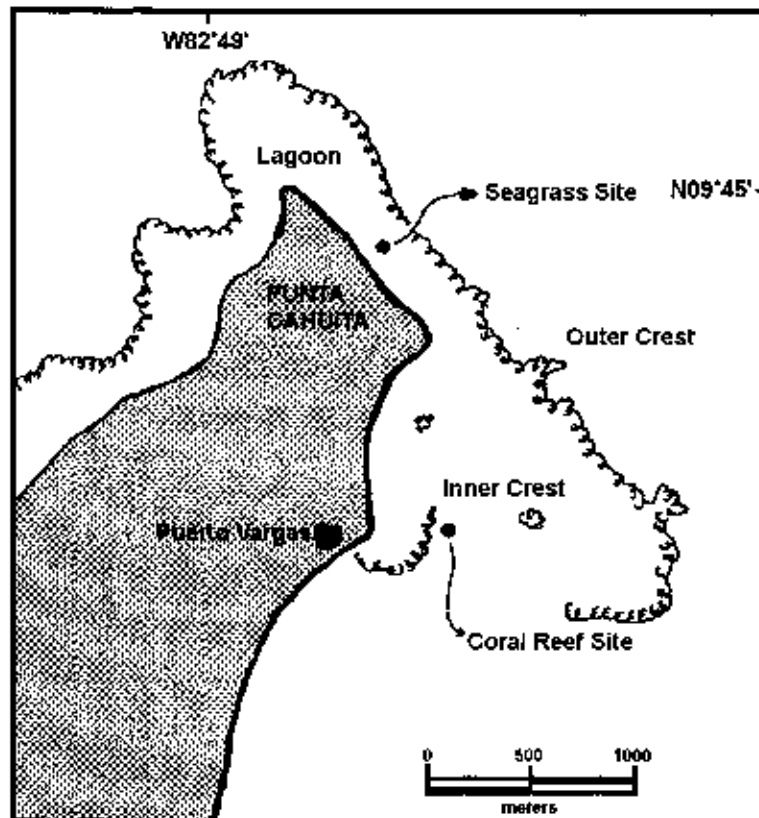
Fig. 3. Seagrass and coral reef sites at Parque Nacional Cahuita, Costa Rica.
