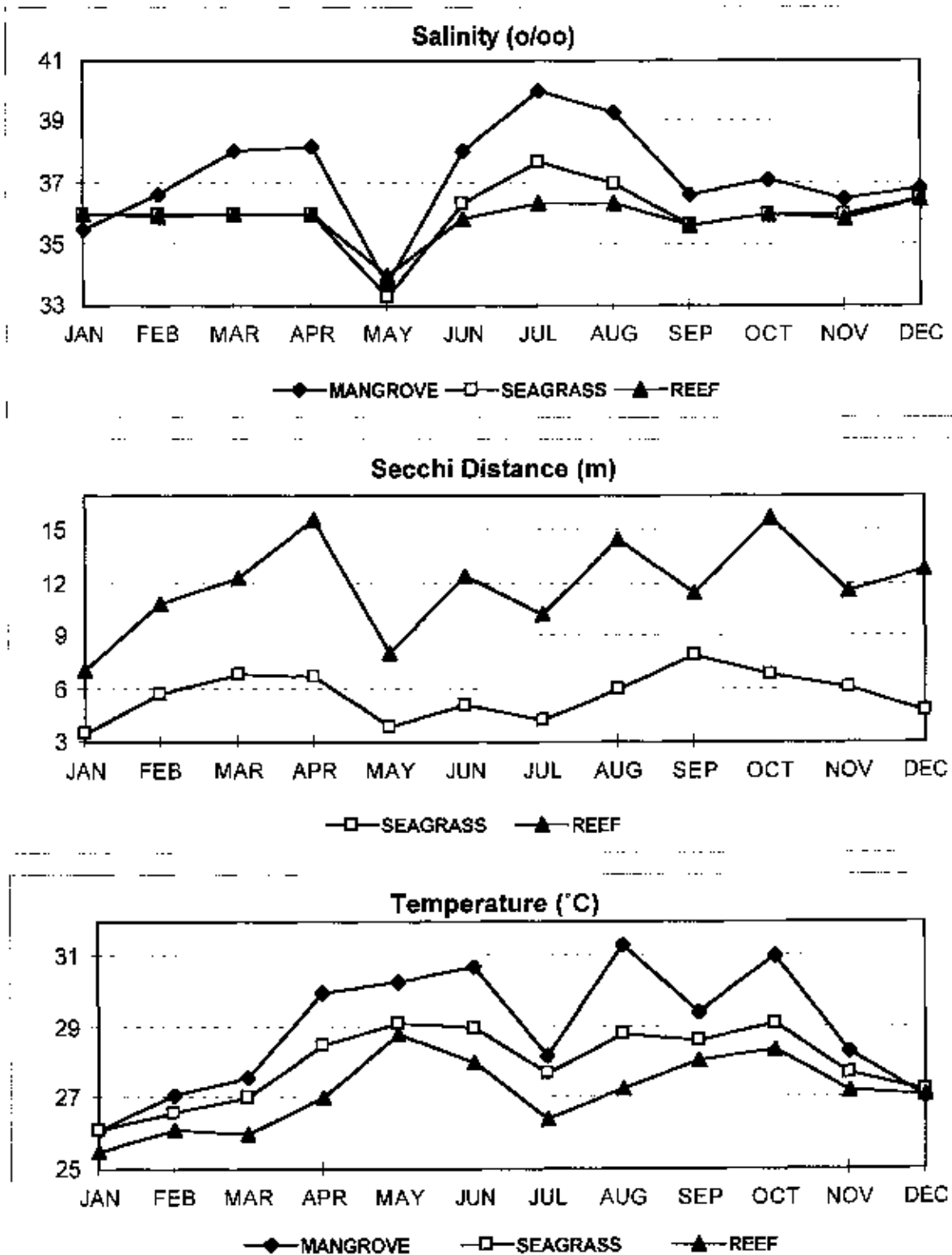
Fig. 3. Mean monthly surface salinity and temperature, and Secchi disk visibility at CARICOMP habitat sites (mangrove wetland, seagrass bed, and coral reef) in Bahía de Chengue during 1993.
