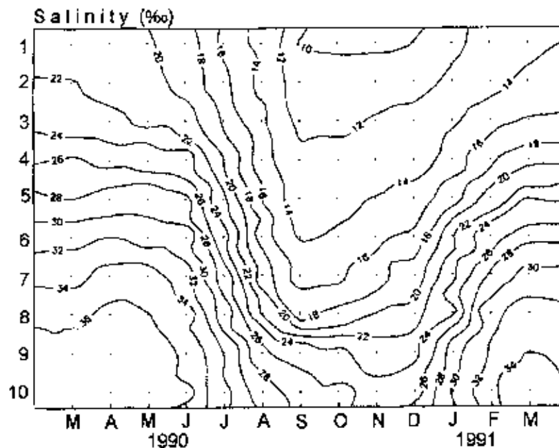
Fig. 3. Space-time diagram of salinity (‰) in Laguna de Celestón during a one-year cycle.
