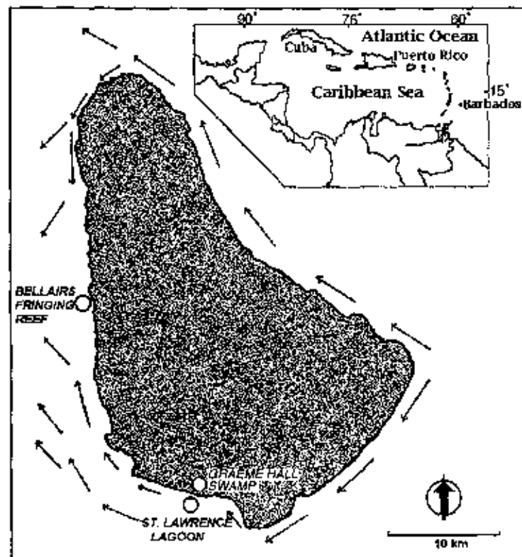
Fig. 1. Map of Barbados with postulated current patterns and locations of CARICOMP sites. (Redrawn from Younglac, 1988; based on studies by Murray et al. , 1977; Peck, 1978).
