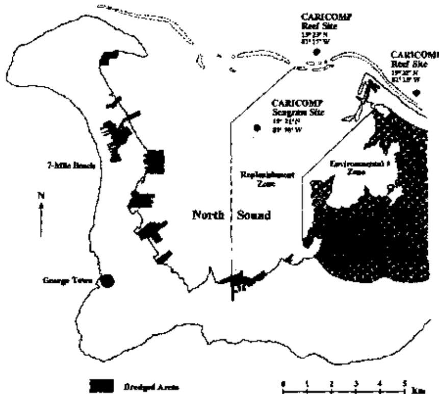
Fig. 3. North Sound, Grand Cayman, showing CARICOMP sites.
