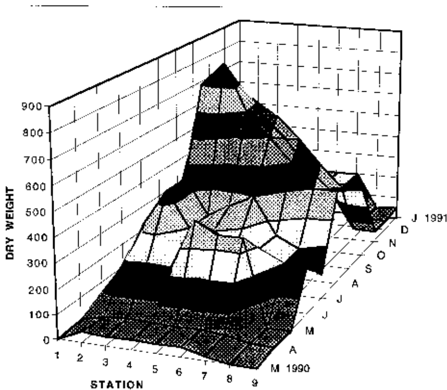
Fig. 5. Mean seasonal changes in the biomass ( \text{g m}^{-2} dry weight) of submerged macrophytes in Laguna de Celestún during a one-year cycle.
