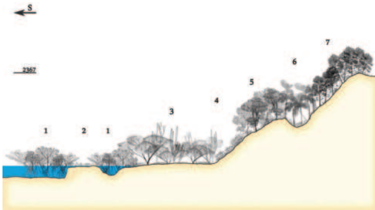
Figure 8. Profile of the vegetation of the cloud forest of Sierra Bahoruco. (1) Rhaddadenio biflori-Laguncularietum racemosae and Lonchocarp pycnophylli-Conocarpetum erecti . (2) Salt marshes of Batidi-Salicornietea . (3) Lonchocarp pycnophylli-Cylindropundietum caribaeae . (4) Melocacto pedernalensis-Leptochloopsietum virgatae . (5) Broad-leaved forest. (6) and (7) Cloud forest of Prestoea montana .
