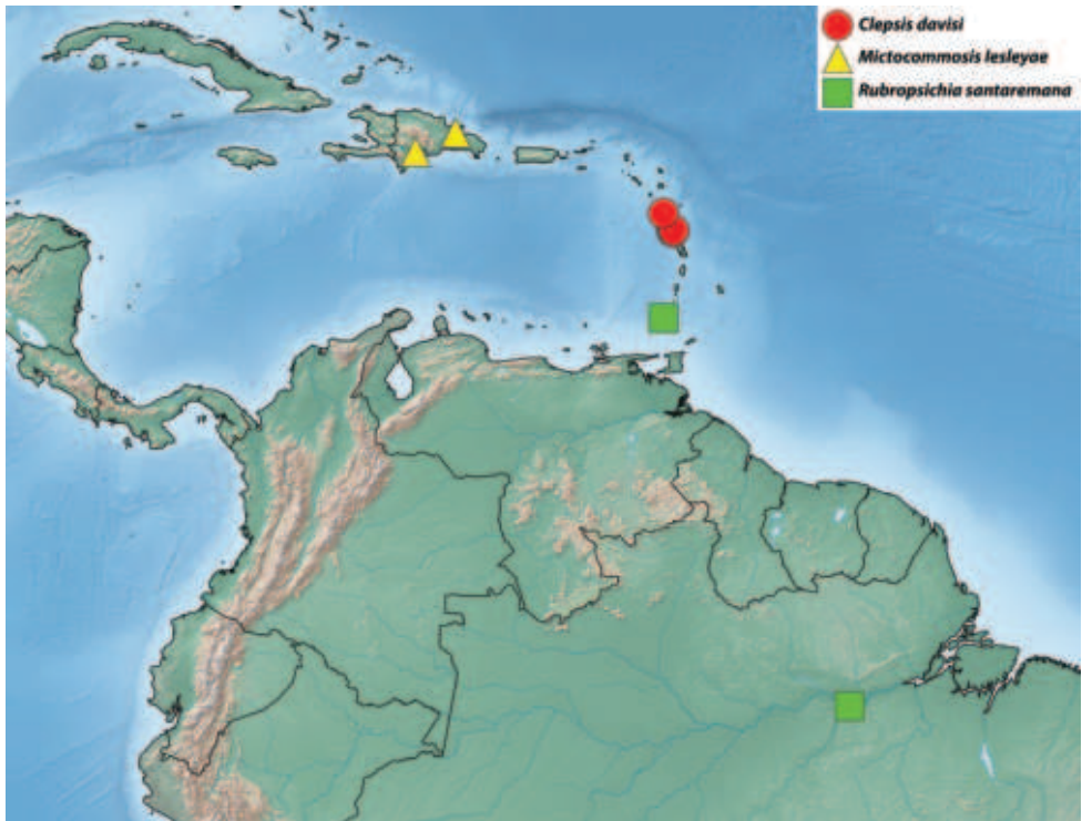
Figure 27. Clepsid , Mictocommosis and Rubropsichia species distributions. Legend inset.
