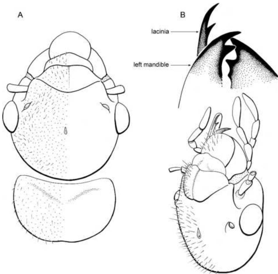
Fig. 9. Heads and pronotum of Anoplotermes spp. in Dominican amber; both are holotypes. A. A. carib , n. sp., dorsal view. AMNH DR10-1541. B. A. maboia , n. sp., dorsolateral view of head (pronotum not fully visible), with detail of mandibles and lacinia. AMNH DR10-1567.
