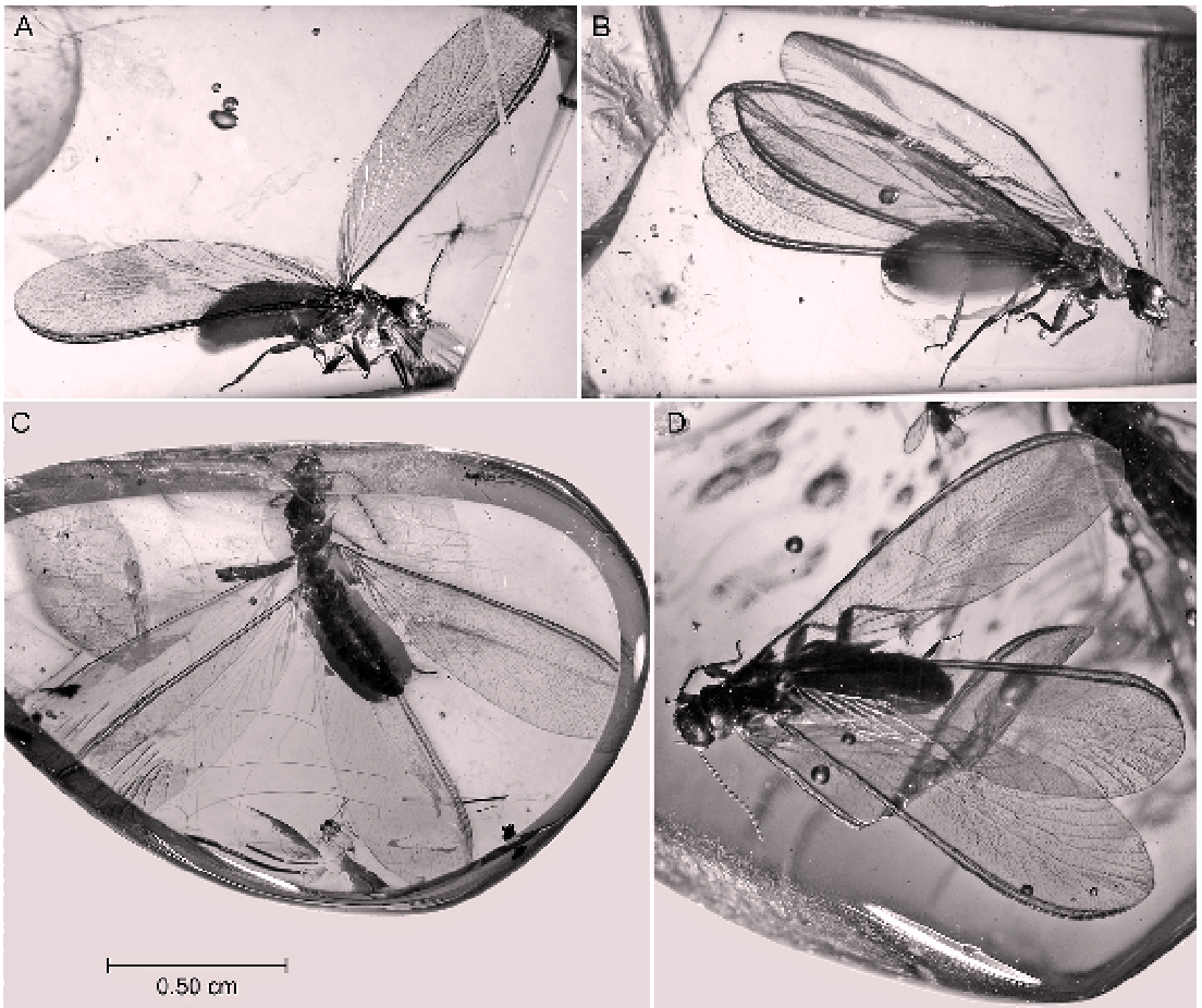
Fig. 1. Photomicrographs of Coptotermes species in Dominican amber. A. Coptotermes hirsutus , n. sp., AMNH DR-PB278. B. Coptotermes hirsutus AMNH DR10-1656. C. Coptotermes paleodominicanus , n. sp., AMNH DR10-1513. D. Coptotermes priscus Emerson, AMNH DR-PB279.
