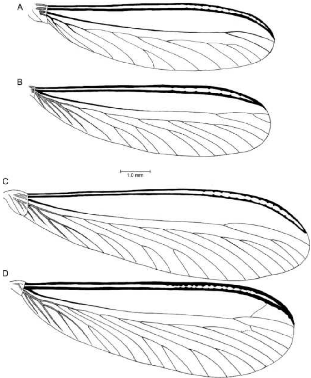
Fig. 3. Wings of Coptotermes species in Dominican amber. A, B. Coptotermes hirsutus , n. sp., AMNH PB278. A. forewing; B. hindwing. C, D. Coptotermes paleodomnicus , n. sp., AMNH DR10-1513.
