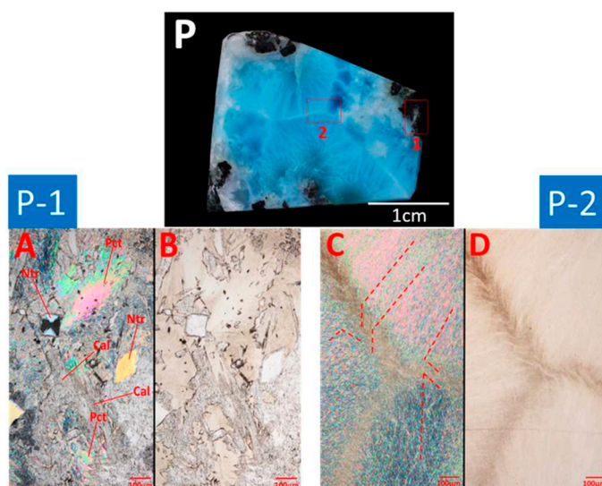
Figure 12. Two thin sections were made from sample P: one is P-1 (photos A and B), near the wall rock, and the other is P-2 (photos C and D), located at the triple junction of white streaks. In P-1, we can observe the symbiosis of the three minerals: pectolite (Pct), calcite (Cal), and natrolite (Ntr). P-2 is mainly composed of fine fibrous pectolite. (Photos A and C: crossed nicol; photos B and D: open nicol.
