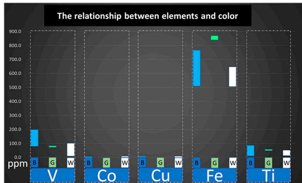
Figure 15. Histogram of Larimar’s color and element correlations. The column-shaped color blocks represent the color of the pectolite: B for blue color, G for green color, and W for white and colorless.
