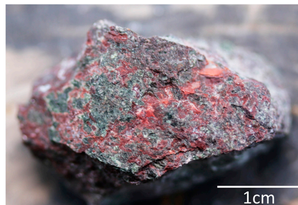
Figure 9. Basalt with hematite mineralization.
