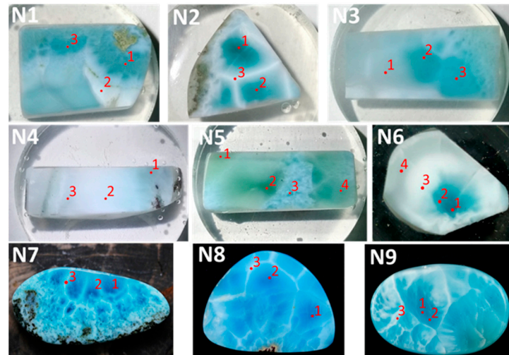
Figure 13. Raman and elemental analysis points of each sample. The number 1, 2, 3 and 4 on the photos means the analyzed position of Micro-Raman and chemical composition.
