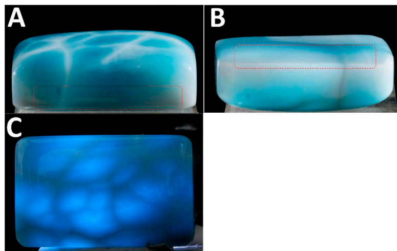
Figure 19. Observing Larimar from different angles; the red square frames in (A,B) are at the same position. However, the original dark-blue color in (A) turned white when it was flipped by 180°. (C) was used for the observation of penetrating light, and the transmittance at the white streaks was low.
