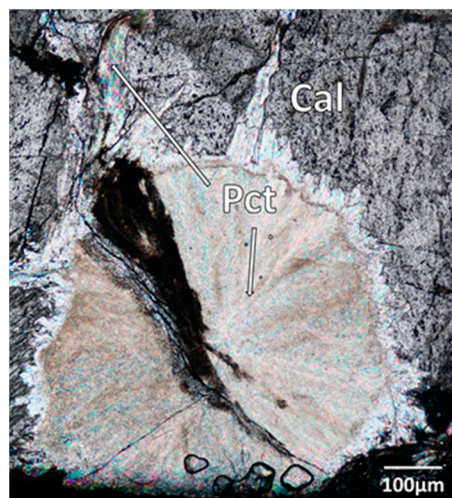
Figure 20. Larimar growing with radial fibers. Pectolite grew later than calcite and penetrated into the cracks of calcite (Pct: pectolite, Cal: calcite).
