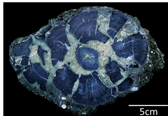
Figure 7. Plant fossil with unapparent Larimar replacement.
