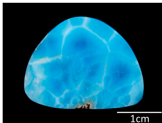
Figure 3. Larimar gem with sea-wave features.
