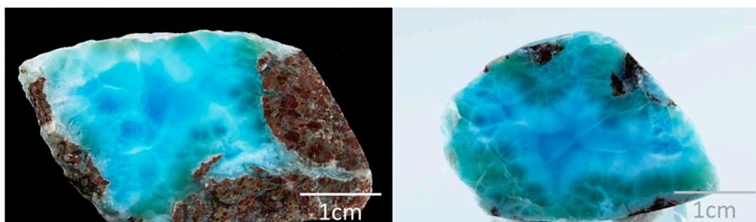
Figure 18. These photos show that green Larimar is distributed almost against the wall rocks.
