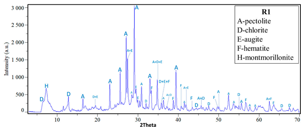
Figure 17. XRD plot of the sample R1.
