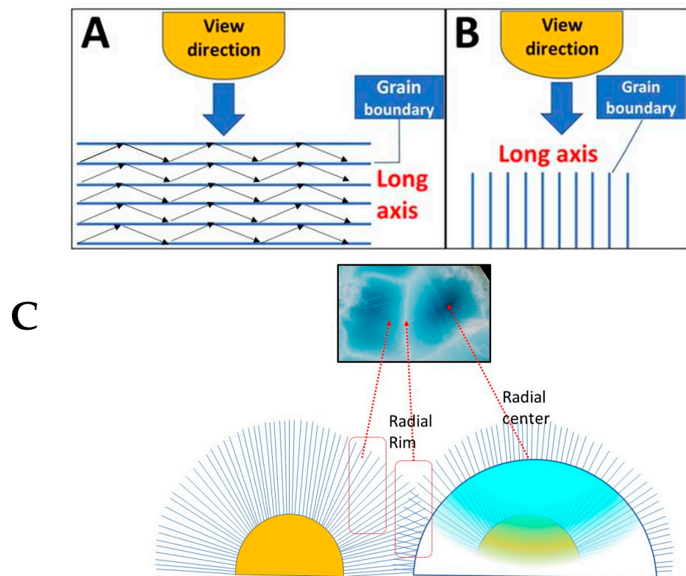
Figure 21. (A) The line of sight is perpendicular to the long axis of the fiber, and more light is reflected to the naked eye, leading to a white color. (B) When the line of sight is parallel to the long axis of the fiber, light passes directly through the crystals to our eyes, and the natural color can be seen. (C) Different directions of the radial ball crystals display a natural color in the cutting center and white reflection at the edge of the crystal boundary.
