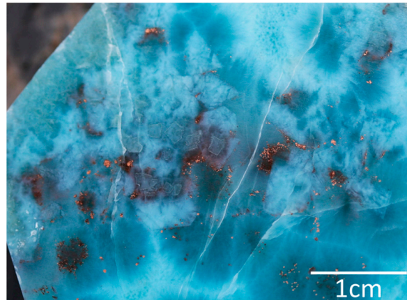
Figure 4. Spots of native copper crystals grown within interstitial Larimar.
