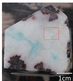
Figure 11. Blue–green pectolite in the interstice of calcite; the red square is the sampling position for U–Th dating. The light-blue pectolite filled in the fissure of calcite.
