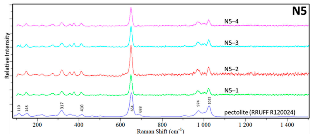
Figure 14. The Raman spectrum of each analysis point in sample N5, all of which were determined to be pectolite after comparison to the RRUFF database.
