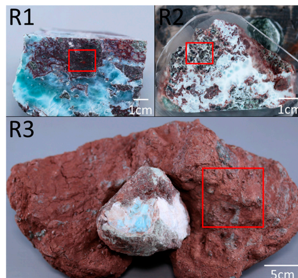
Figure 16. Sample photos of wall rocks R1, R2, and laterite R3. The red rectangle is sampling area.
